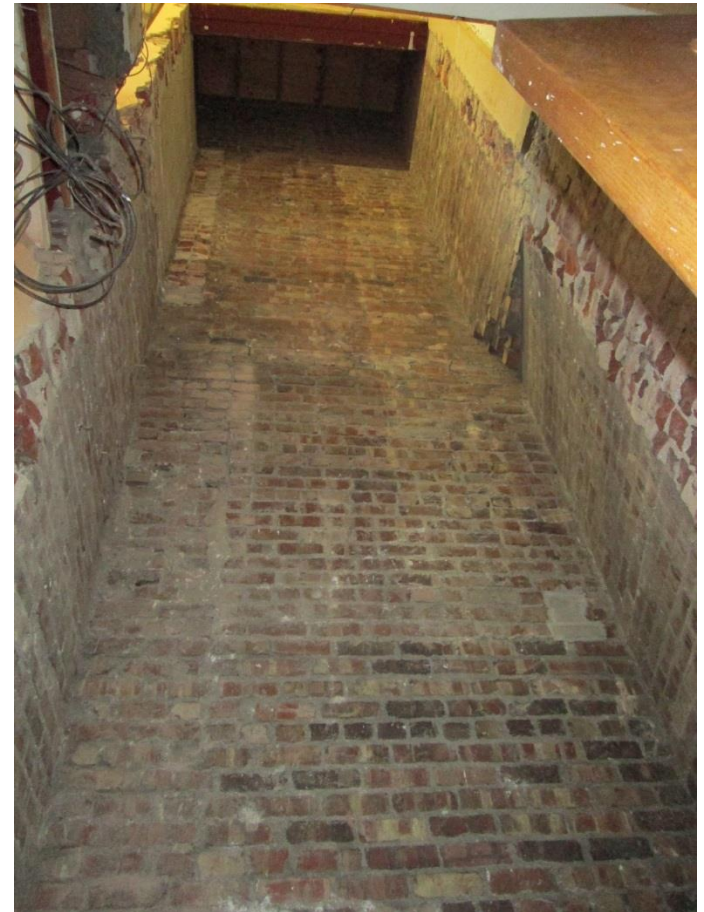
Hoistway for new elevator in existing stair shaft
